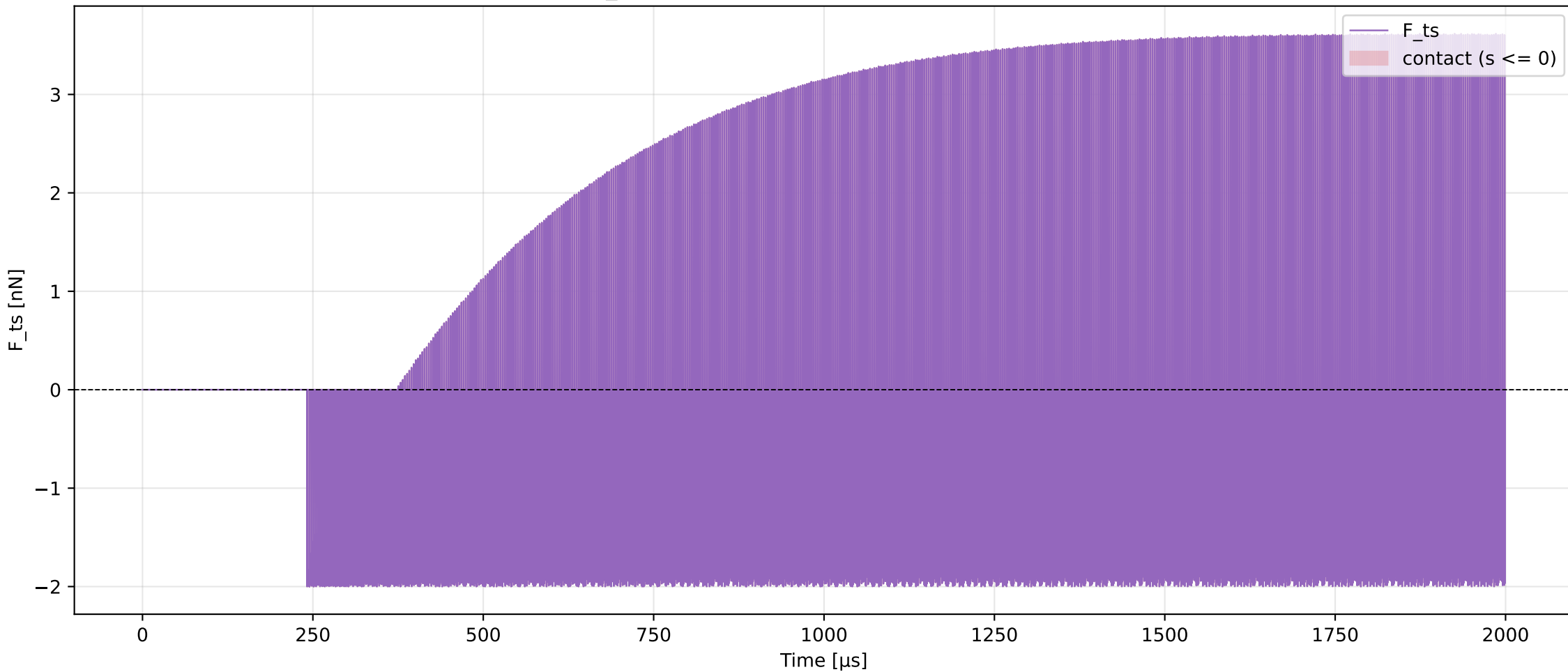
AFM DMT-KV F ts Time-Domain Signal (hard contact, no smoothing)
